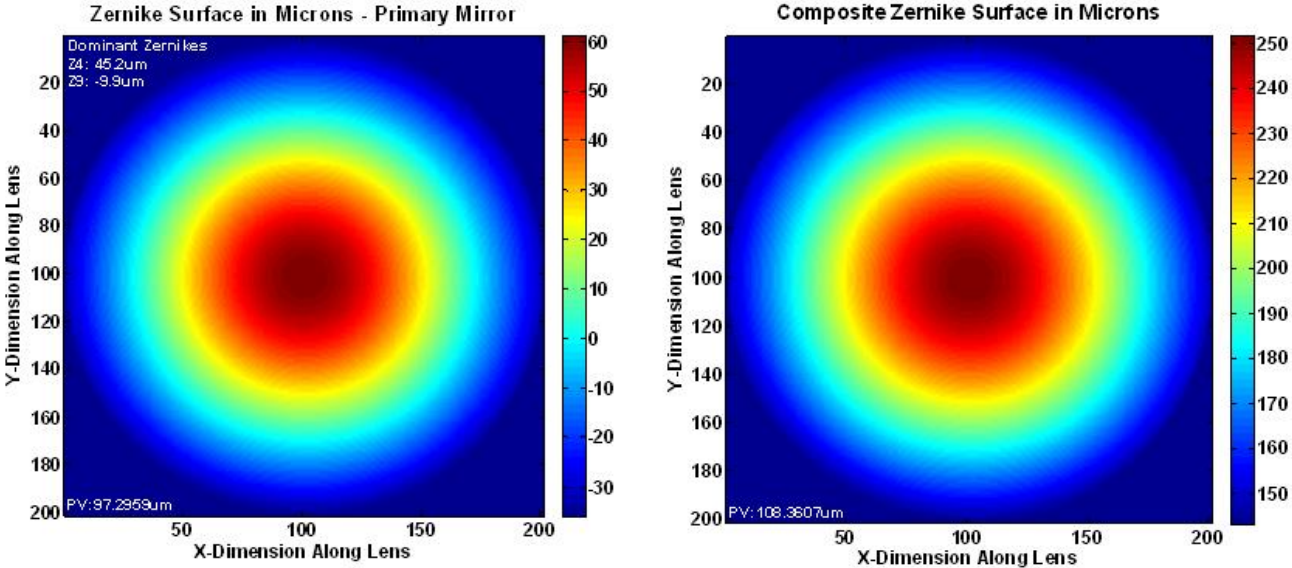
Figure 9: Wavefront and surface height error predictions
